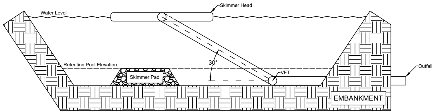
Elevation View
