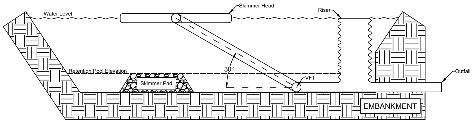
Elevation View
